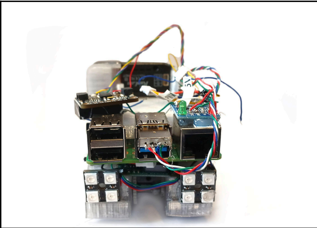
Picture 2: Back view
