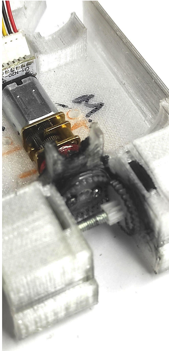
Picture 21: Drive motor and transfer gear fully assembled and tested
