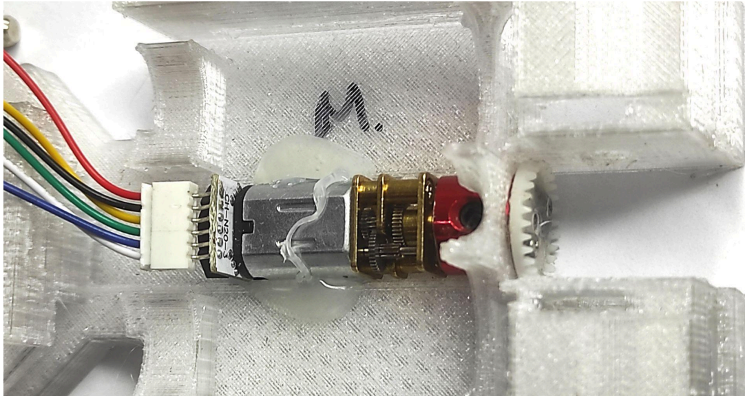
Picture 16: Motor and gearbox fitted in frame
