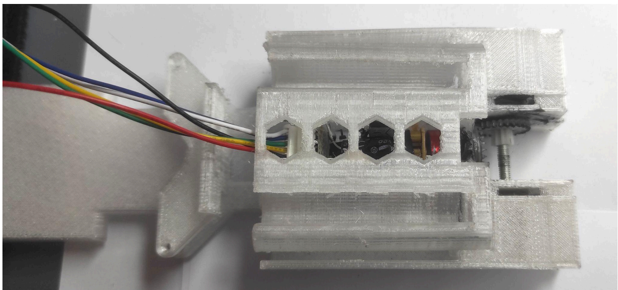
Picture 26: Motor driver and drive system fully assembled and enclosed with housing
