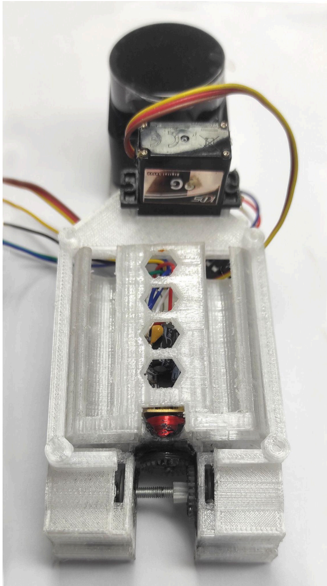
Picture 27: Steering servo and LiDAR placed
