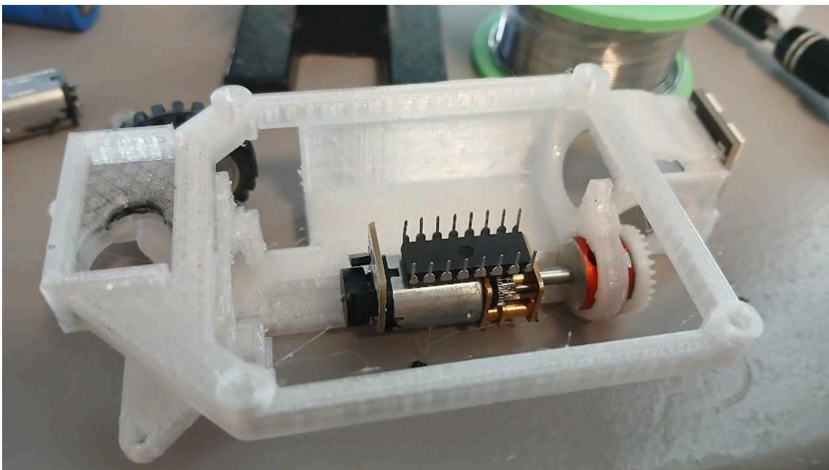
Picture 11: Motor driver mounted upside-down in demonstration frame
