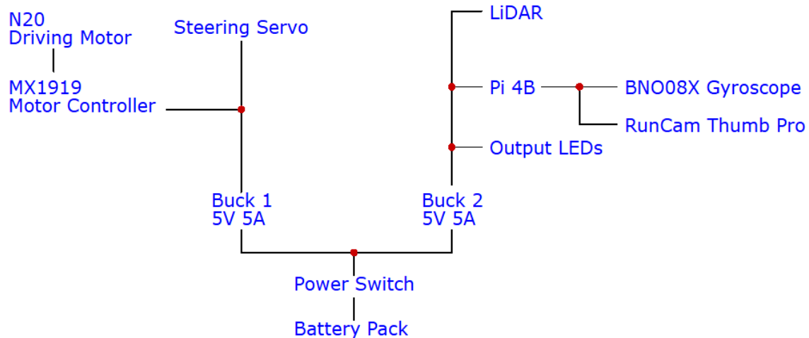
Diagram 11: Power Distribution map
