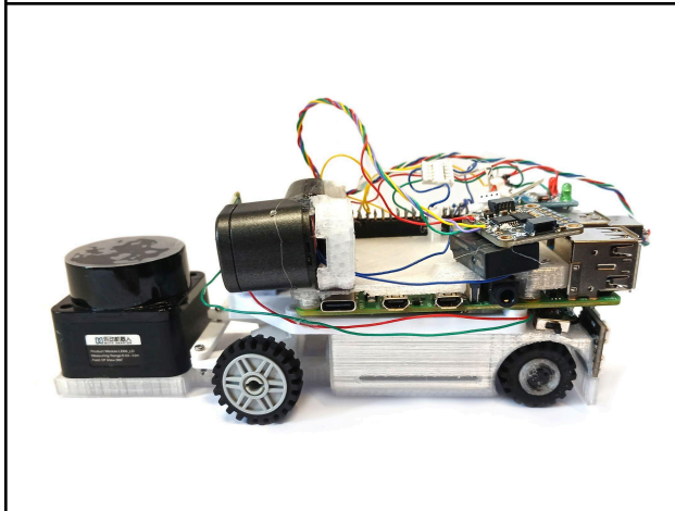
Picture 3: Left side view
