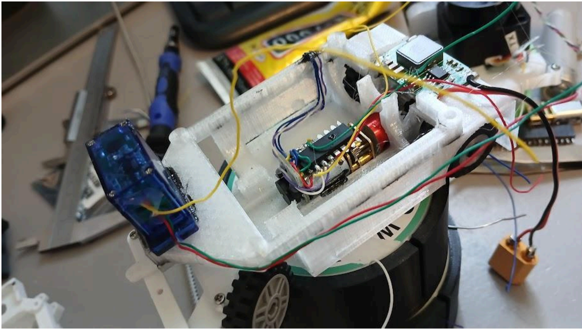
Picture 10: Wires soldered to the motor driver
