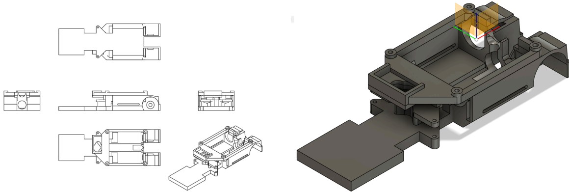
Diagrams 9 & 10: Blueprint for main frame
