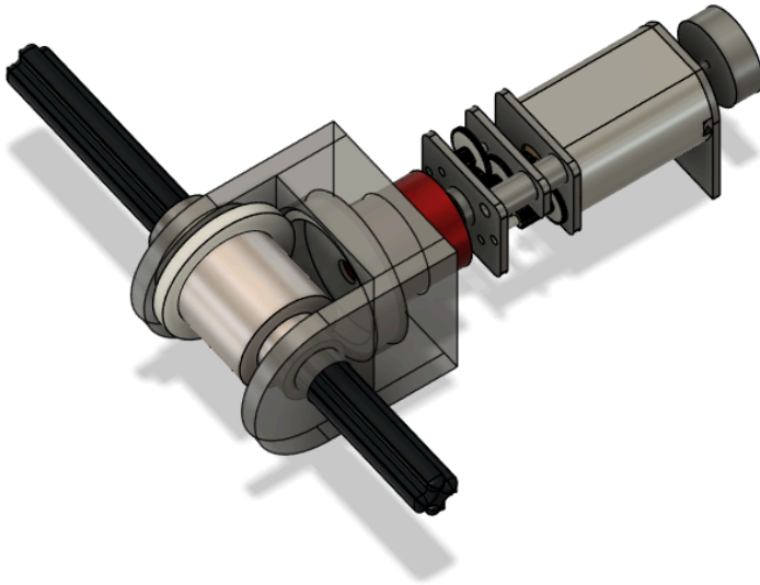
Diagram 3: CAD Model of the complete motor-gearbox-axle assembly
