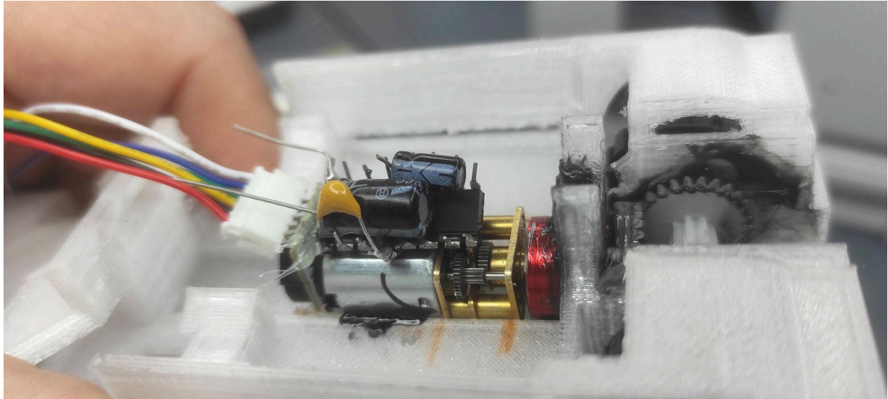
Picture 25: Motor driver and motor assembled into a single conjoined unit
