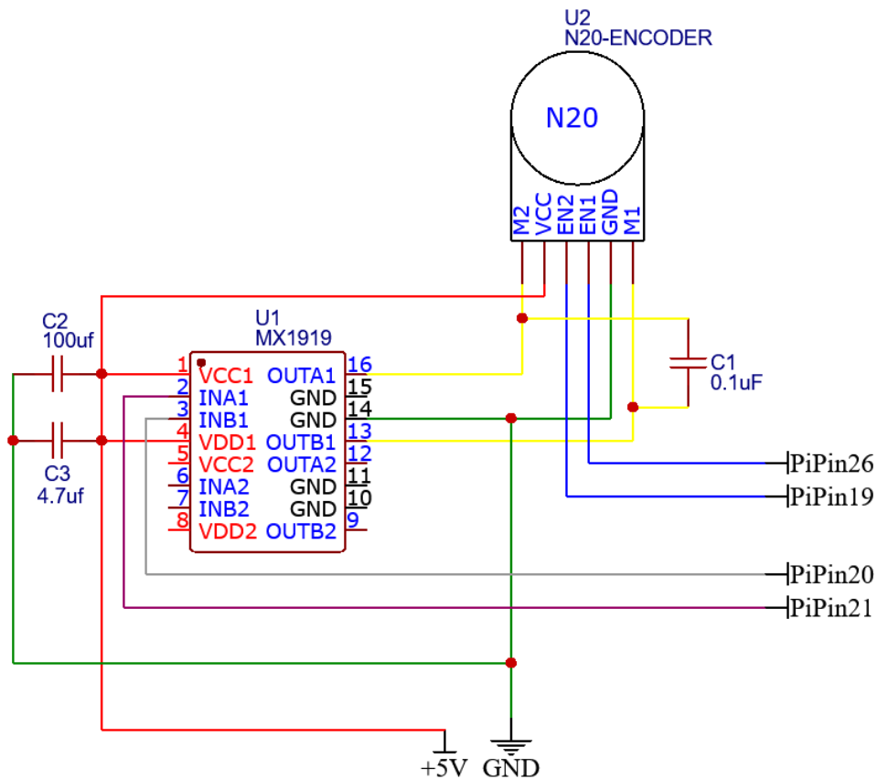
Diagram 5: Schematic for motor driver
