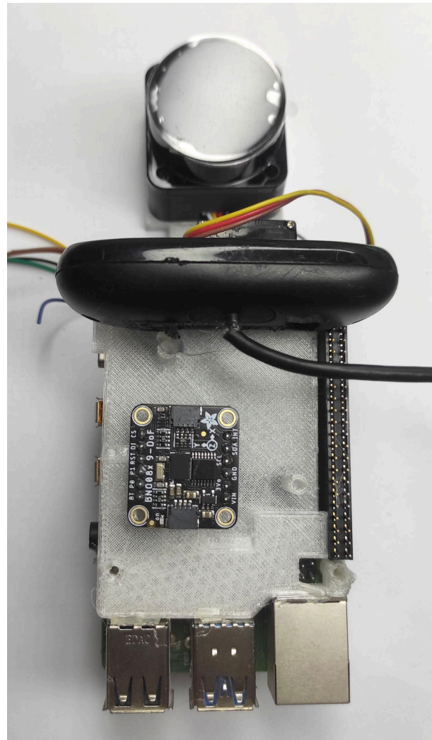
Picture 30: Gyroscope and camera fitted
